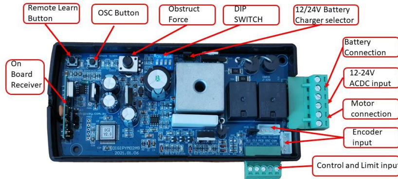
Digiway SL300
